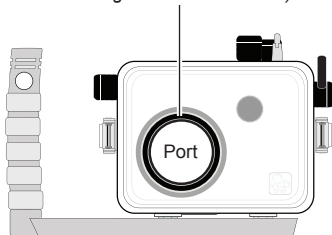
Diagram C O-ring Seal (view from rear of housing with back removed)
